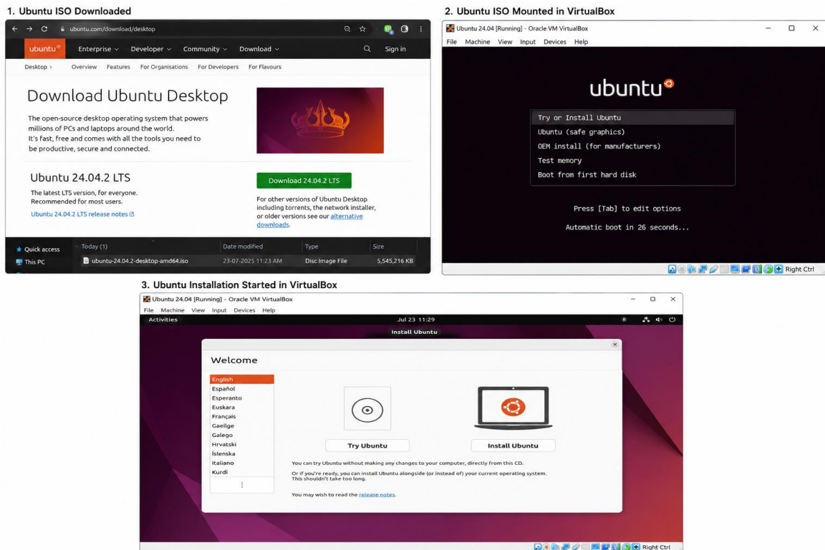
Fig 2. Ubuntu Installation
